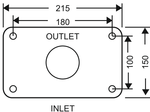
PUMP BASE
